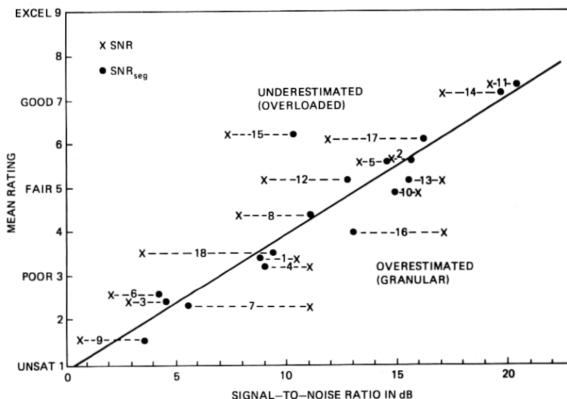
Fig. 10—Mean ratings for the 18 coders vs. SNRs showing the improvement in prediction by measuring SNR_{seg} segmentally. The solid line is the graph of formula 2, Table III, the regression of rating on SNR_{seg} .
